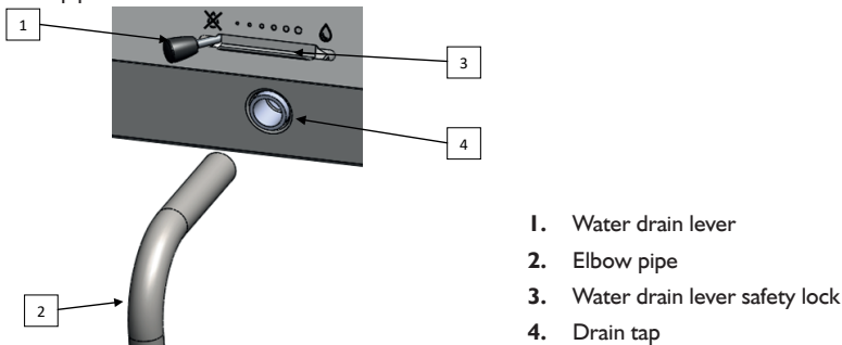
Figure 9. Elements of the water drain mechanism
