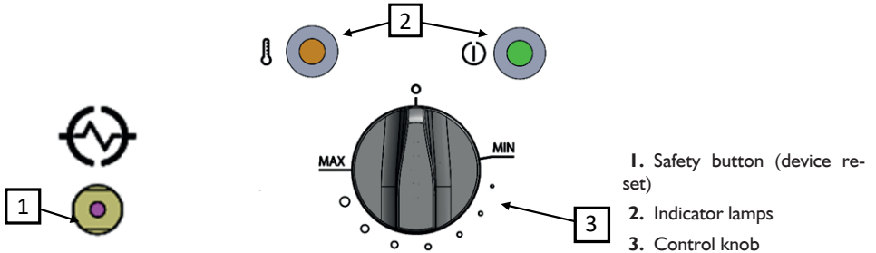
Figure 8. Control elements of the device
